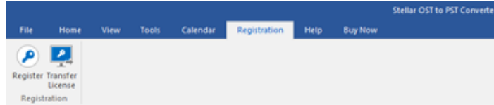
Registration Menu
