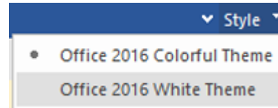
Style Menu
