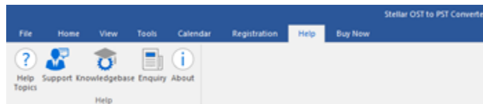
Help Menu
