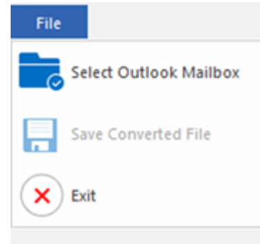
File Menu
