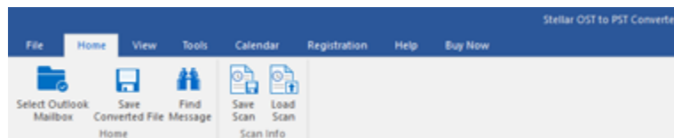
Home Menu
